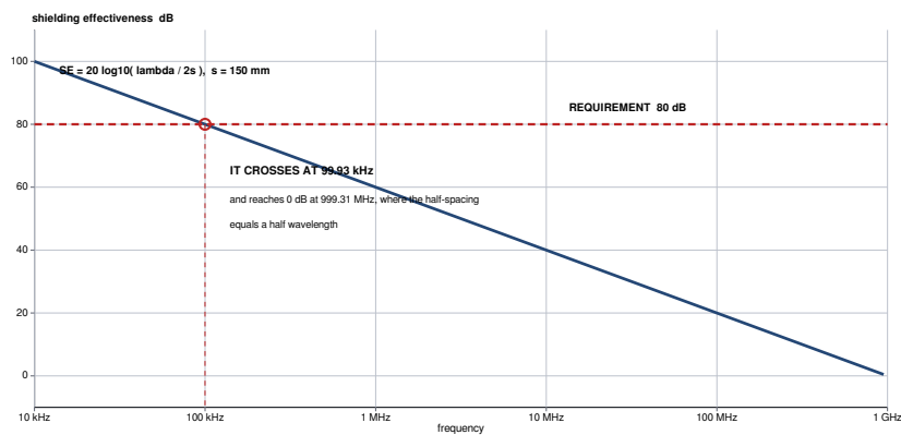
SHIELDING EFFECTIVENESS OF THE 150 mm REINFORCEMENT CAGE
