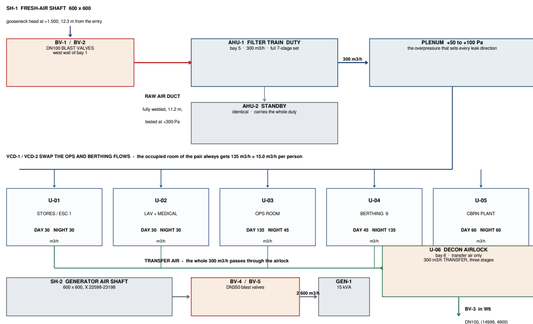
VENTILATION AIR PATH AND ROOM DISTRIBUTION
