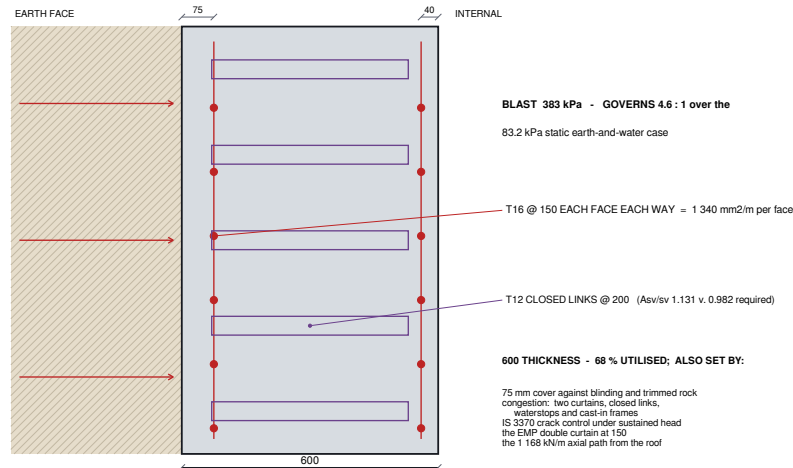
Fig 7.1 : Perimeter wall W1 to W4, section and reinforcement
