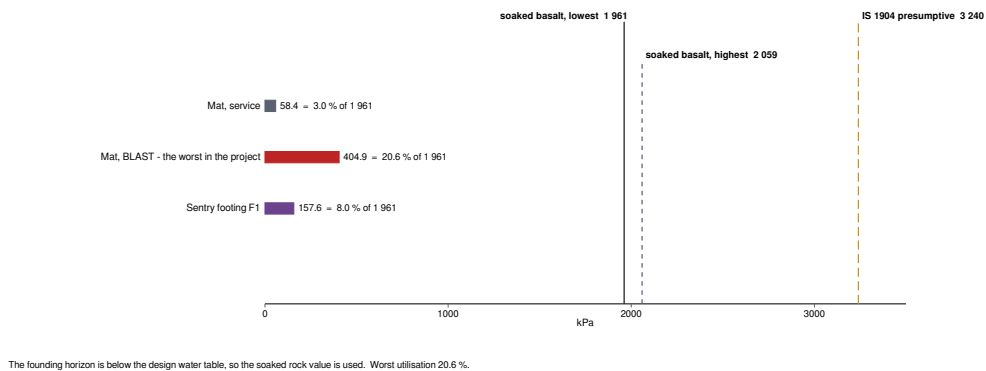
Fig 2.7 : Bearing demand against capacity
